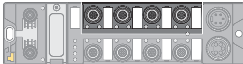
Abb. 21: M12-Steckverbinder, IO-Link-Master-Ports, Class A
