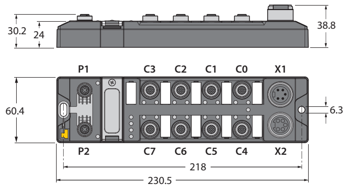
Abb. 5: Abmessungen TBEN-L5-8IOL
